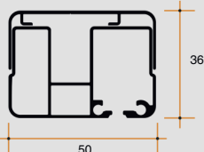
Estetika® by Clearline Motorized Telescopic Guide
